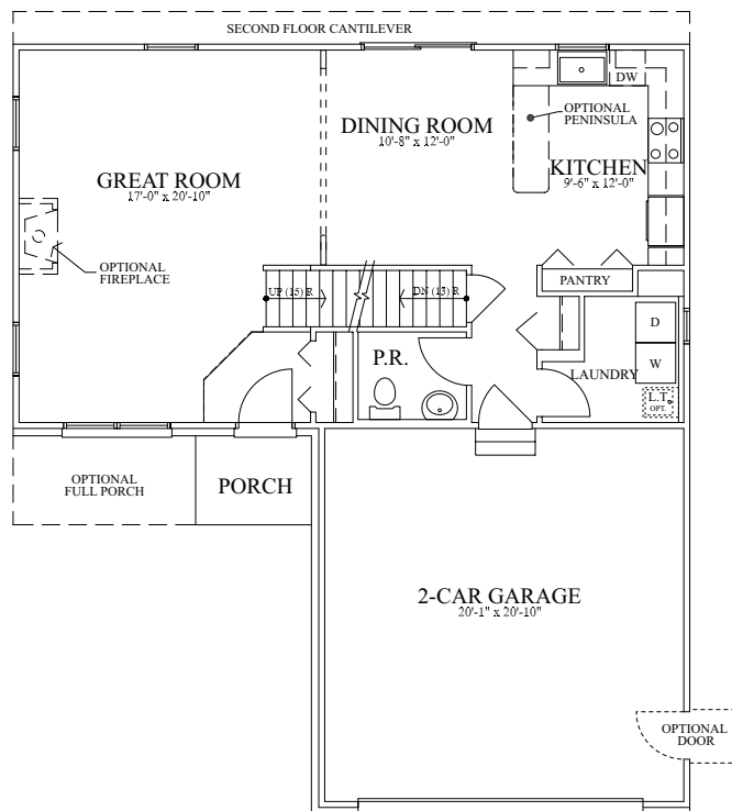
MAIN FLOOR
