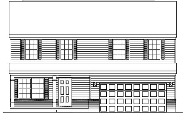
ELEVATION II
