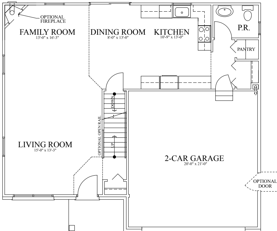
MAIN FLOOR
