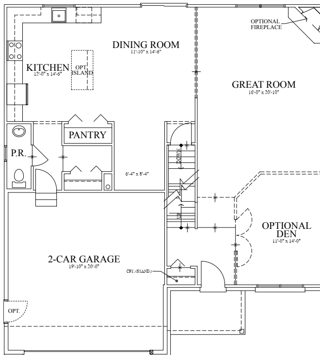
MAIN FLOOR
